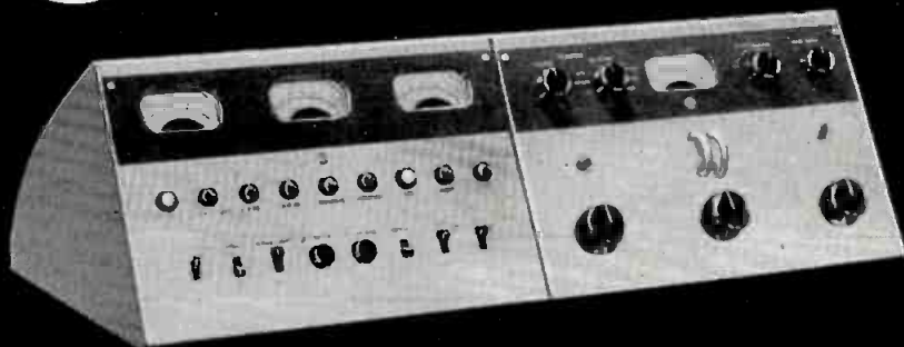
BTC-1B TRANSMITTER CONTROL CONSOLE. Handles all audio mixing and transmitter switching for AM station operation. Add-a-unit design does away with obsolescence—enables you to add control turrets and desk sections as your station grows.
