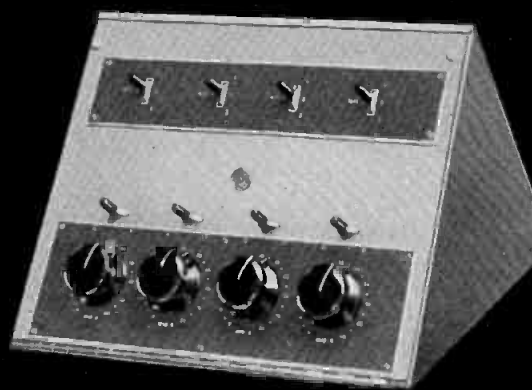
BCM-1A AUXILIARY MIXER CONSOLE. For large AM and TV studios. It triples the microphone inputs of the BC-2B—up to 16 microphones can be connected—8 can be used simultaneously. Enables you to "block-build" as required.
